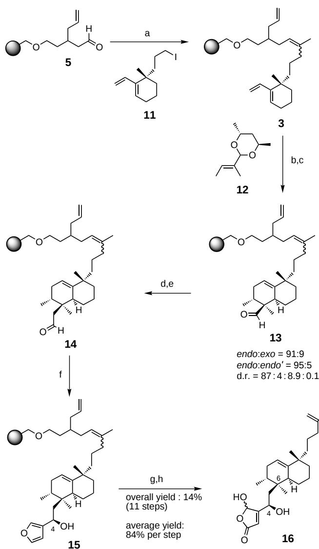
Scheme 3. Solid-phase synthesis of 16 . Reagents and conditions: a) \text{EtP-Ph}_3\text{I} , n\text{BuLi} , 11 , THF, RT, 16 h, then n\text{BuLi} , 0^\circ\text{C} , 2 h; b) trimethylsilyltri-fluoromethanesulfonate, dichloromethane, -78^\circ\text{C} , 7 h; c) p -toluenesulfonic acid, acetone, dichloroethane, \text{H}_2\text{O} , \Delta , 20 h; d) \text{Ph}_3\text{PCH}_2\text{OMeCl} , \text{KOtBu} , THF, RT, 4 h; e) pyridinium p -toluene sulfonate, THF, \text{H}_2\text{O} (1%), \Delta , 16 h; f) 3-bromofuran, n\text{BuLi} , THF, -78^\circ\text{C} , 5 h; g) \text{O}_2 , \text{EtPr}_2\text{N} , rose bengal, h\nu , dichloromethane, -78^\circ\text{C} , 5 h, then RT, 10 min; h) (\text{PCy}_3)_2\text{Cl}_2\text{-Ru=CHPh} ( 2 \times 10\text{ Mol \%} ), dichloromethane, RT, 16 h.
